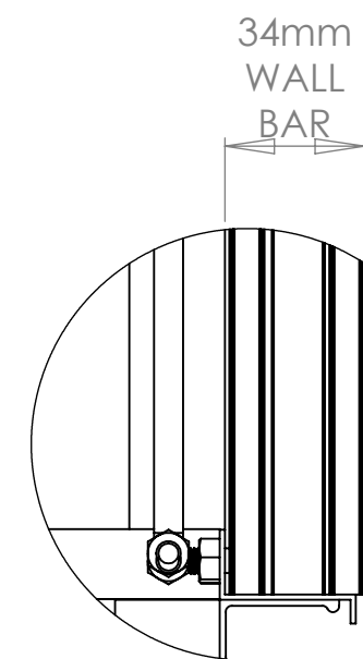
DETAIL A SCALE 1 : 2
